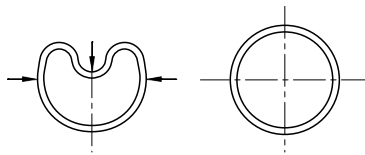
Fig. 4.11 Slipper Seal®, rod-type, installation 2
